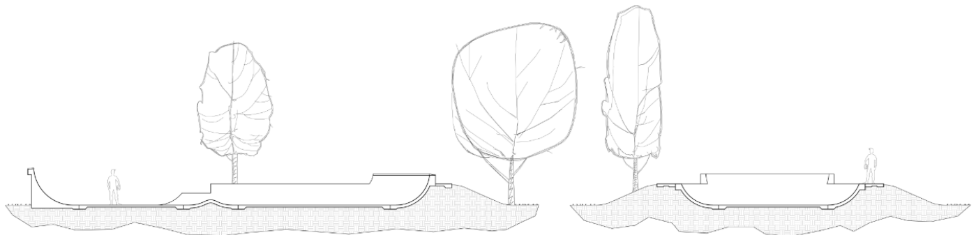
C SECTION 3/8" = 1'-0"
